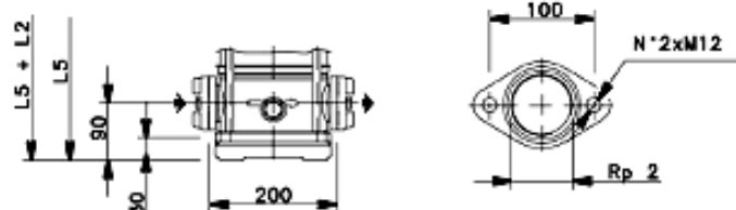
50-15 T DN(50)
