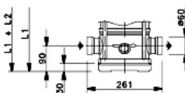
50-15 V DN(50)
