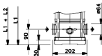
50-15 C DN(50)
