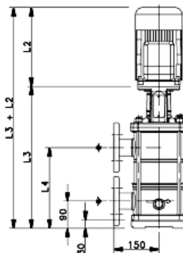
50-15 T DN(50)
